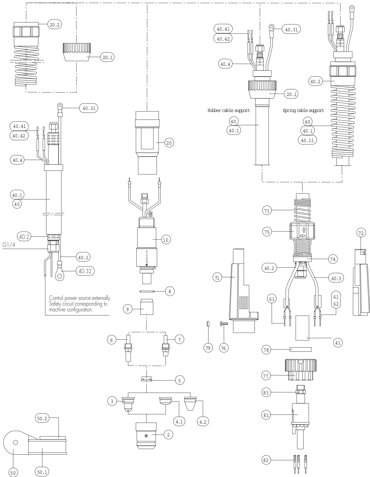
Single connector
